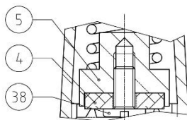
480 / AU480 / 480BP / AU480BP : DN08 to 25
