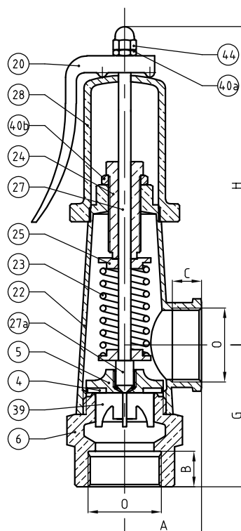
Ref. 479.Ø, 479BPØ and 479TØ DN40 and DN50
