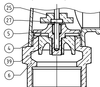
Ref. 479.Ø, 479BPØ and 479TØ DN65 and DN80
