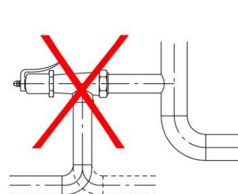
Montage incorrect
