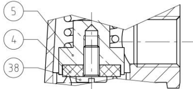
481 / AU481 / 481S / AU481S: DN08 to 25
