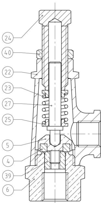
481T / AU481T: DN08 to 15 & 80 481.80 / AU481.80 / 481S80 / AU481S80
