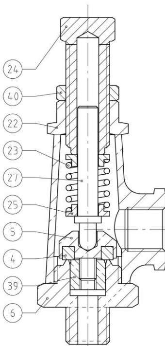
281 / AU281: DN08 to 15 & 80 381.80 / AU381.80 / 381S80 / AU381S80
